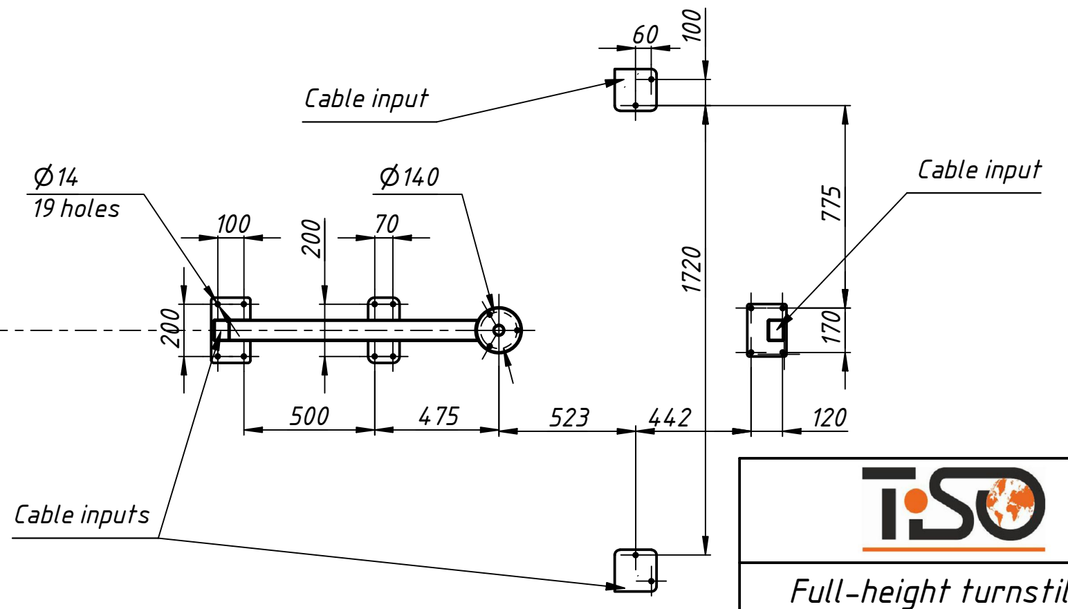
Installation template
